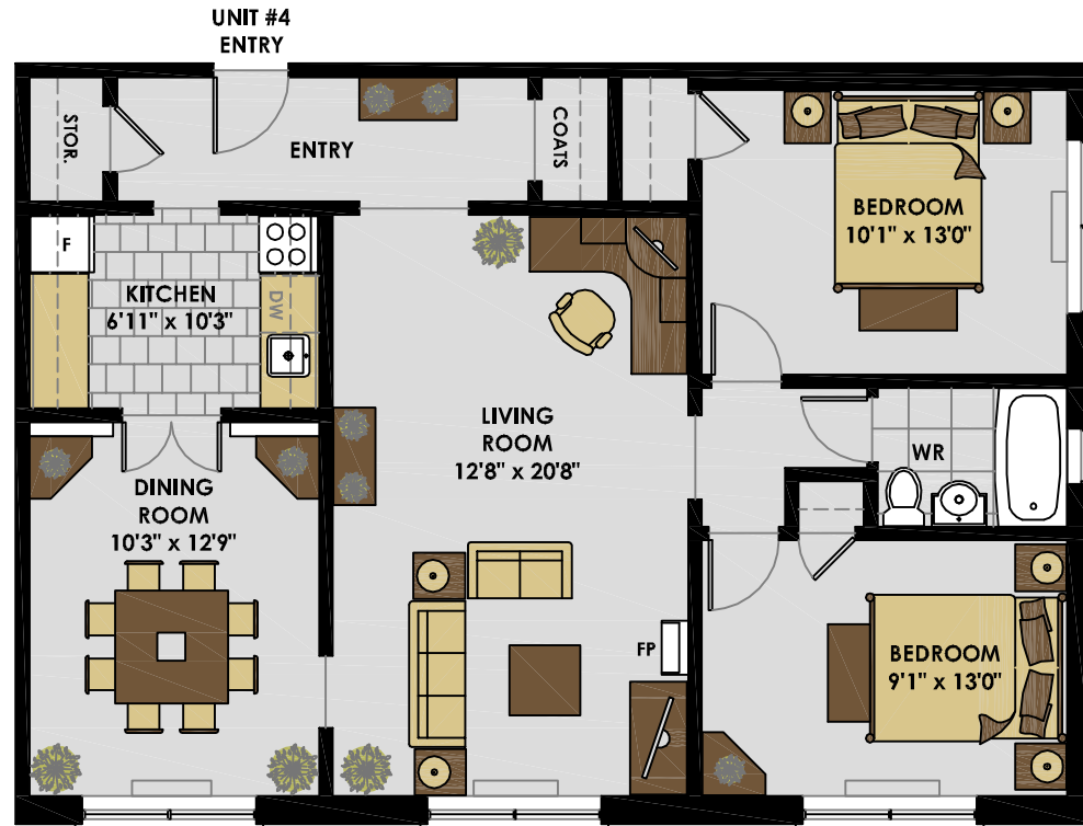
GROUND FLOOR PLAN UNIT #4 (Approx. 1,015 s.f.)
